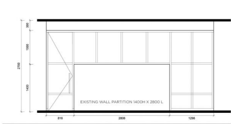
NEW MEETING ROOM WALL DETAIL
