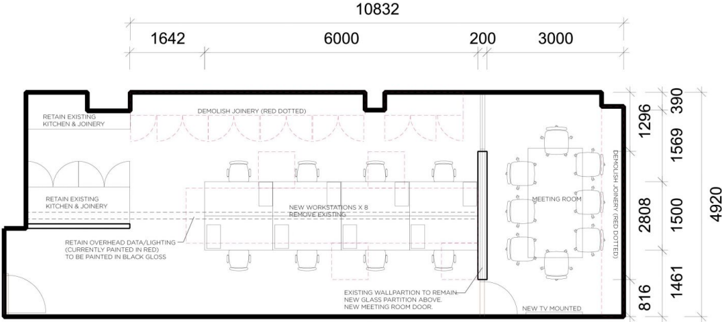
PROPOSED WORKS
